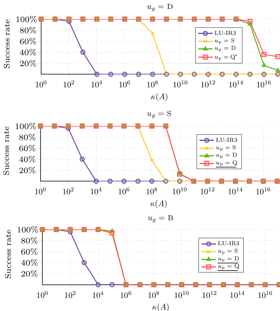
FIG. 4.1. Proportion of matrices for which LU-IR3 and GMRES-IR5 with varying u_p and u_g converged to double precision forward error as a function of \kappa(A) . For all variants, u_f = B , u = D , and u_r = Q . The underlined terms denote combinations of precisions that are not meaningful in Table 3.3. The GMRES-IR5 variant with an asterisk “*” is equivalent to GMRES-IR3. (Color available online.)
