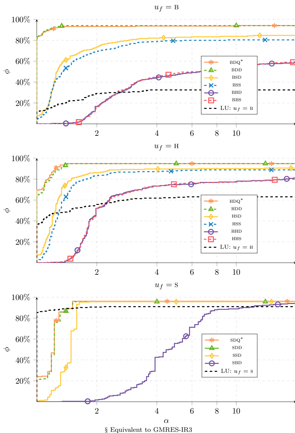
FIG. 4.3. Performance profile of LU-IR3 and GMRES-IR5 variants (with u_f, u_g, u_p as specified in the legend) on 230 SuiteSparse matrices. \phi (y-axis) indicates the percentage of matrices for which a given variant requires less than \alpha (x-axis) times the number of LU solves required by the best variant. GMRES-IR5 variants with an asterisk "*" are equivalent to GMRES-IR3 variants.
